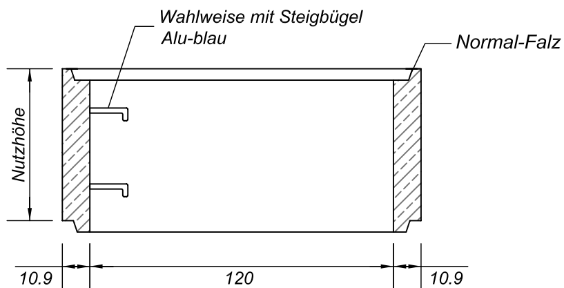
PIMA-Schachtring
